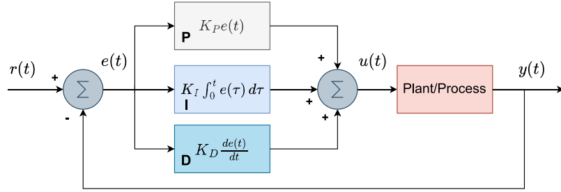
Fig. 4. Block diagram of the PID control loop showing error computation, proportional-integral-derivative actions, and feedback correction.
