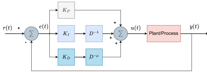
Fig. 5. Block diagram of fractional-order and variable-order PID controllers. In the VOPID, the fractional orders vary as \lambda = \lambda(t) and \mu = \mu(t) .
