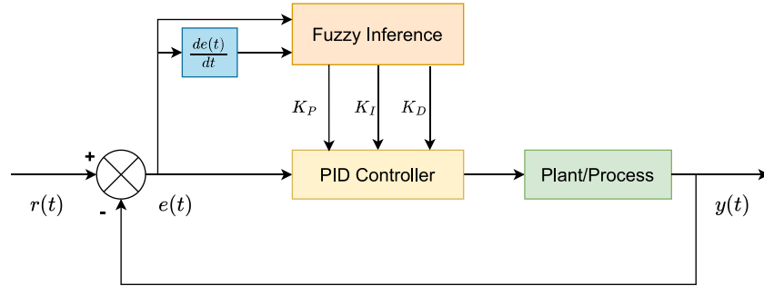
Fig. 7. Block diagram of Fuzzy Adaptive PID controller.
