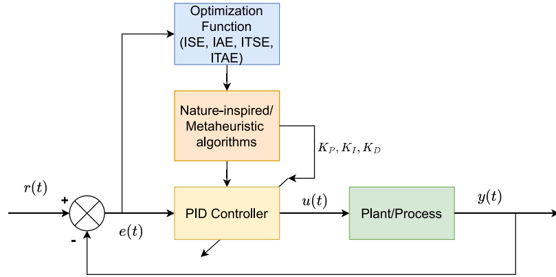
Fig. 6. Block diagram of Nature-inspired/Metaheuristic PID controller.
