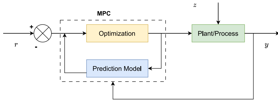
Fig. 8. Basic architecture of an MPC. The controller uses a prediction model and an online optimization routine to compute the constrained optimal input u , which is applied to the plant.
